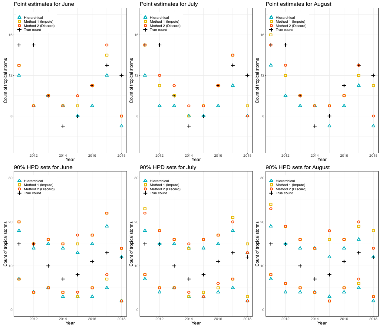
Figure 3: Top panel: Plots showing the observed and predicted (based on medians) counts of tropical storms over 2011-2018. Bottom panel: Plots showing the observed counts of tropical storms over 2011-2018, and endpoints of associated 90% prediction (HPD) sets.
