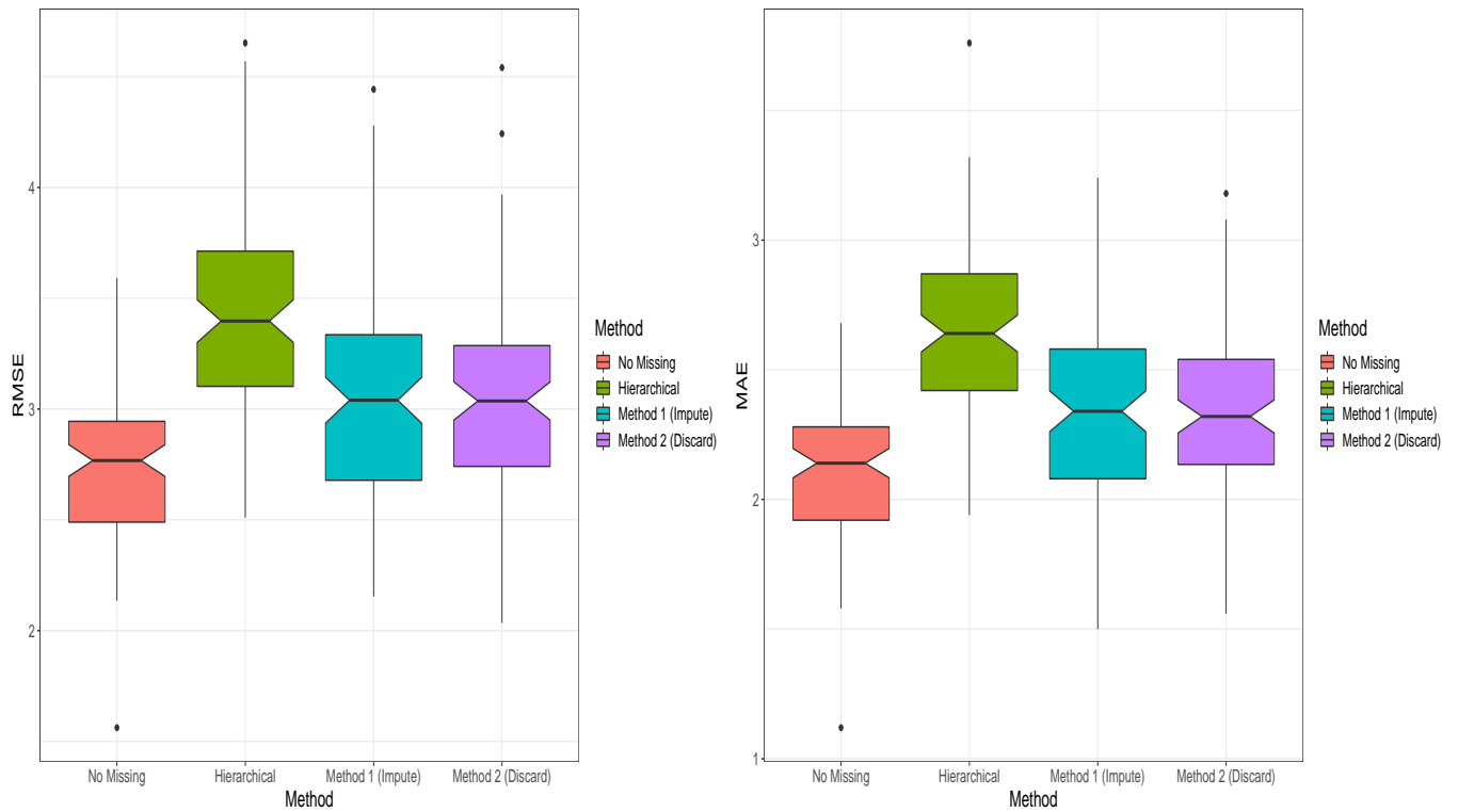
Figure 2: Scenario 2: Notched box plots showing RMSE/MAE of each method; results are shown for 100 datasets.
