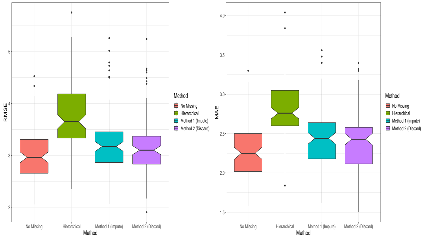
Figure 1: Scenario 1 : Notched box plots showing RMSE/MAE of each method; results are shown for 100 datasets.
